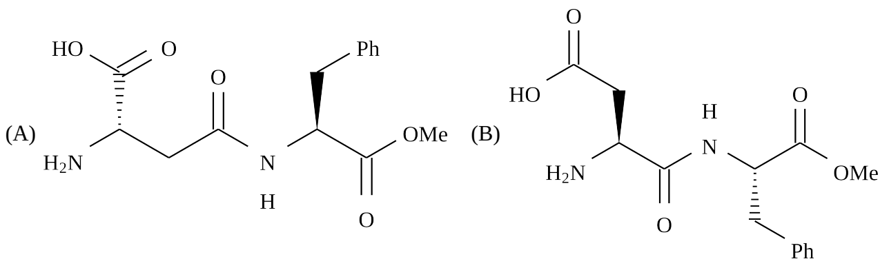
Phenylalanine
