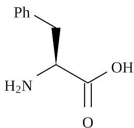
Phenylalanine
