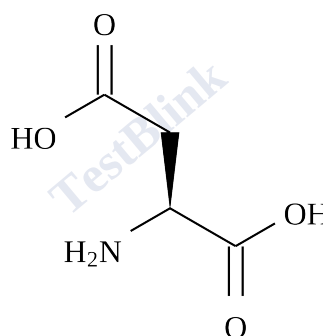
Aspartic acid
